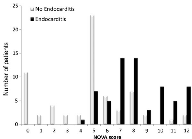
Figure 3. Patients with and without enterococcal endocarditis distributed according to the score in our case-control study (50% endocarditis and 50% no endocarditis). The score was as follows: heart murmur, 1 point; prior valve disease, 2 points; unknown source of bacteremia, 4 points; and continuous bacteremia, 5 points. Abbreviation: NOVA, Number of positive blood cultures, Origin of the bacteremia, previous Valve disease, Auscultation of heart murmur.
