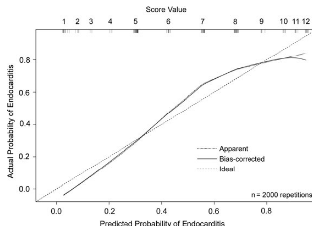
Figure 2. Model calibration curve for predicting enterococcal endocarditis based on the 12-point score obtained by bootstrapping the case-control population. The curve replicates the 4.3% prevalence of infective endocarditis observed in the prospective cohort. Values and number of cases in the original case-control dataset for each score value are shown on the top horizontal axis. Notice that a false-negative diagnosis (actual probability > predicted probability) is not expected for a Number of positive blood cultures, Origin of the bacteremia, previous Valve disease, Auscultation of heart murmur (NOVA) score <4 points.
